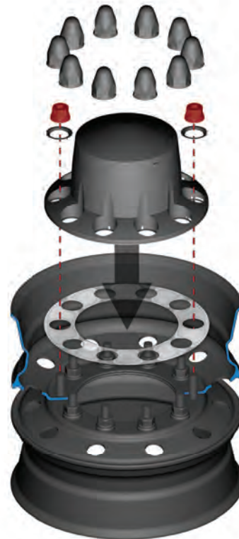
Push-On
