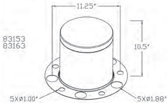
Removable Cap
